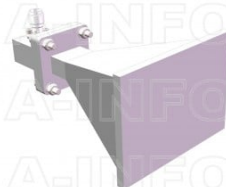
LB-90-15-C-TFSP0 Standard Gain Horn Antenna 8.2-12.4GHz 15dB Gain TNC Female
